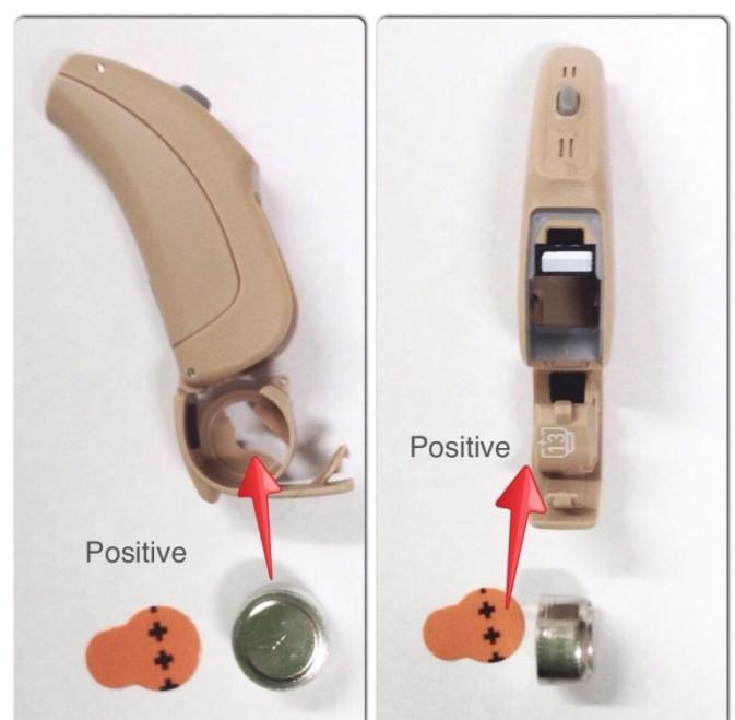
Phonak Nathos S+ Micro – Top & Side View
